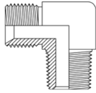
Male BSP x Male BSPT 90° Elbow
