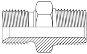
Male BSPP x Male NPT
