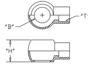
Metric Solder Banjo
