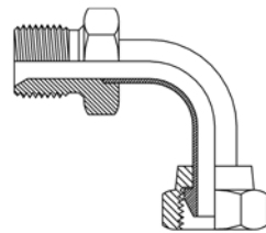
Male BSP x Female BSPP Swivel 90° Elbow
