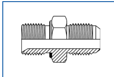
Male BSPP with Seal x Male JIC
