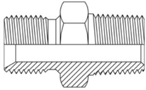
Male Metric x Male NPT
