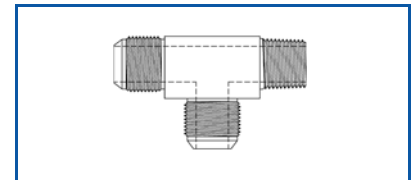
BSPT x JIC Run Tee
