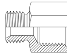
Male BSPP x Female SAE O-Ring
