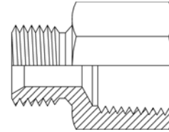
Male Metric x Female NPT
