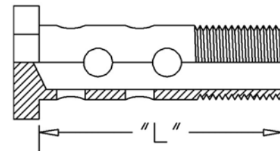
Double Banjo Bolt
