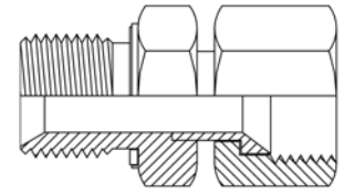
Male Metric with Seal x Female JIC Swivel
