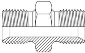
Male BSPP x Male BSPP Nipple
