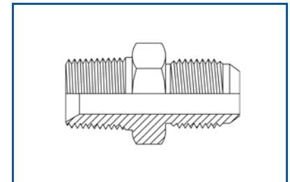
Male BSPT x Male JIC
