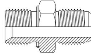
Male Metric with Seal x Male JIC
