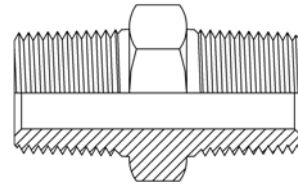
Male BSPT x Male BSPT Nipple
