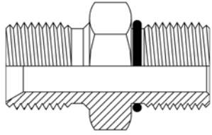
Male BSPP x Male SAE O-Ring
