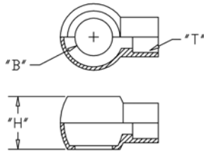
BSPP Solder Banjo
