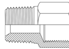
Female BSPP x Male NPT
