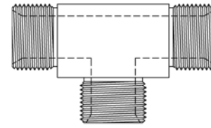
Male BSP Tee
