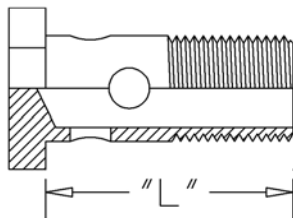
Single Banjo Bolt
