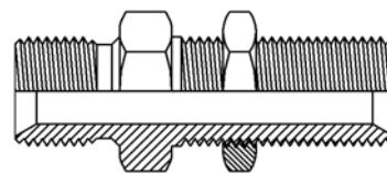
Male BSPP x Male BSPP Bulkhead
