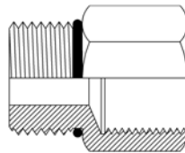
Female BSPP x Male SAE O-Ring
