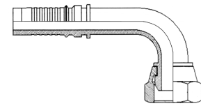
Female BSPP 90° Interlock
