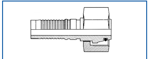
Female DIN2353 Interlock
