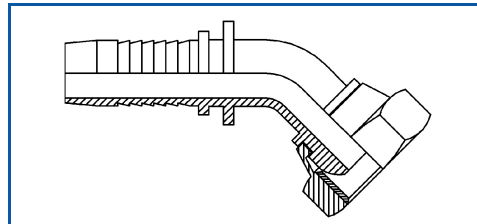
BSP Swivel Female 45° Elbow
