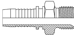
BSPP Male 60° Cone
