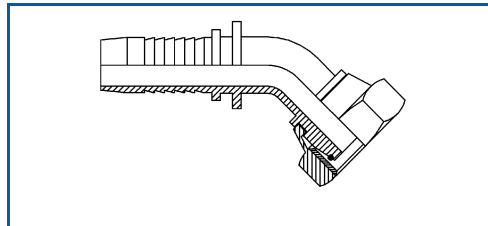
Female Swivel 24° 45° Elbow & O-Ring
