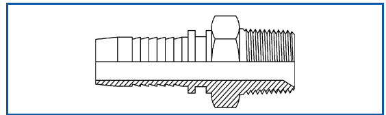
BSPT Male Tapered BSPT Thread Model Number Part Number
