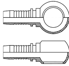
Banjo Hose End
