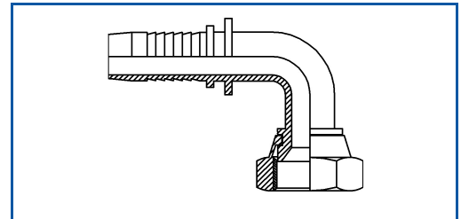
Female JIC 90°
