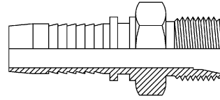
Metric Male 24°
