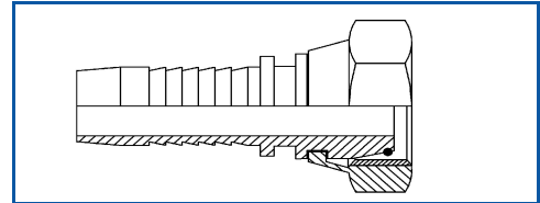
Female Swivel 24° with O-Ring
