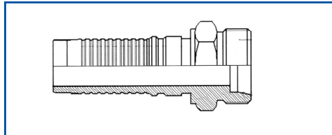
Male DIN2353 S Series Interlock
