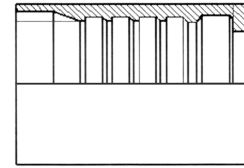
Crimp Ferrule 100R13 Hose Interlock
