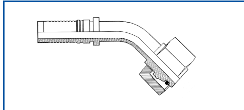
Female DIN2353 45° Interlock
