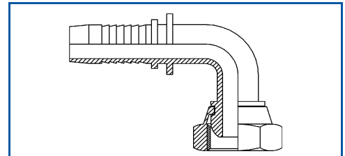
BSP Swivel Female 90° Elbow
