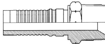
Male NPT Interlock
