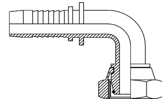
Female Swivel 24° 90° Elbow & O-Ring
