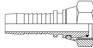
Female Swivel 24° with O-Ring
