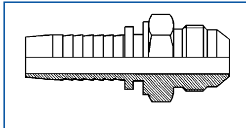
Male JIC
