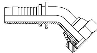
Female Swivel 24° 45° Elbow & O-Ring
