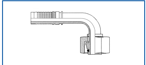
Female DIN2353 90° Interlock
