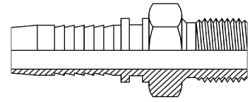
BSPP Male Flat Seat
