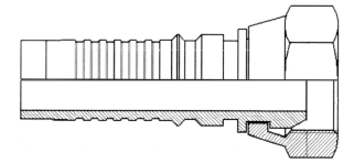
Female BSPP Interlock
