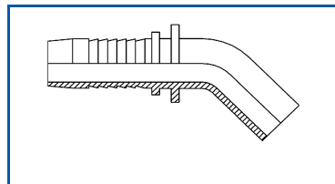
Metric Standpipe 45° Elbow
