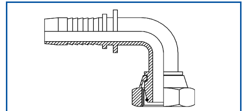
Female Swivel 24° 90° Elbow & O-Ring
