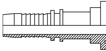
Code 61 Flange
