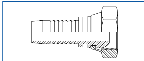
BSP Swivel Female
