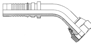
Female BSPP 45° Interlock
