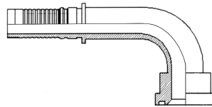
Code 62 Flange 90° Interlock
