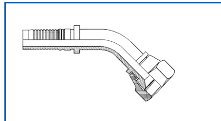
Female JIC 45° Interlock
