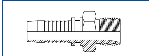
Metric Male 24°
