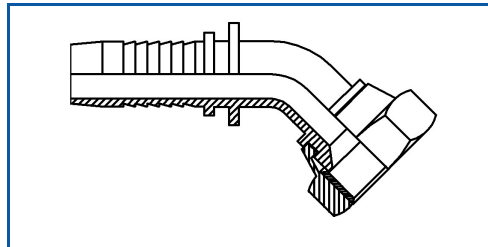
Female JIC 45°
