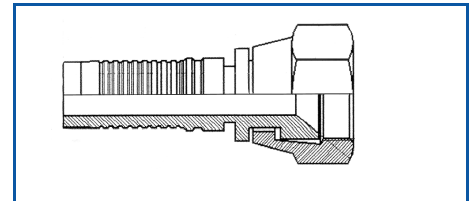
Female JIC Interlock
