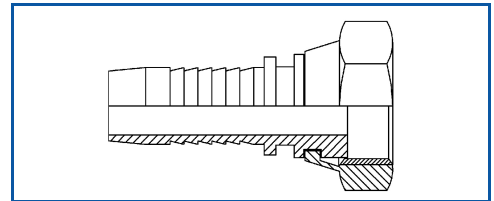
BSP Swivel Female Flat Seat
