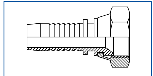
Female JIC
