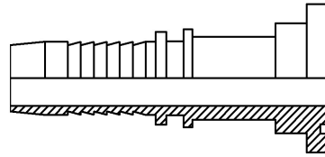
Code 62 Flange
